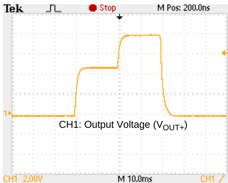
Figure 4. Waveform Showing Detection Pulse into Open-Circuit
